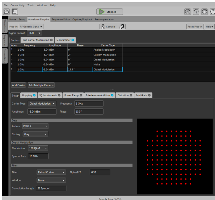
Figure 1: The AWG70000B with the RF Generic Plugin allows complex RF Waveform Generation
