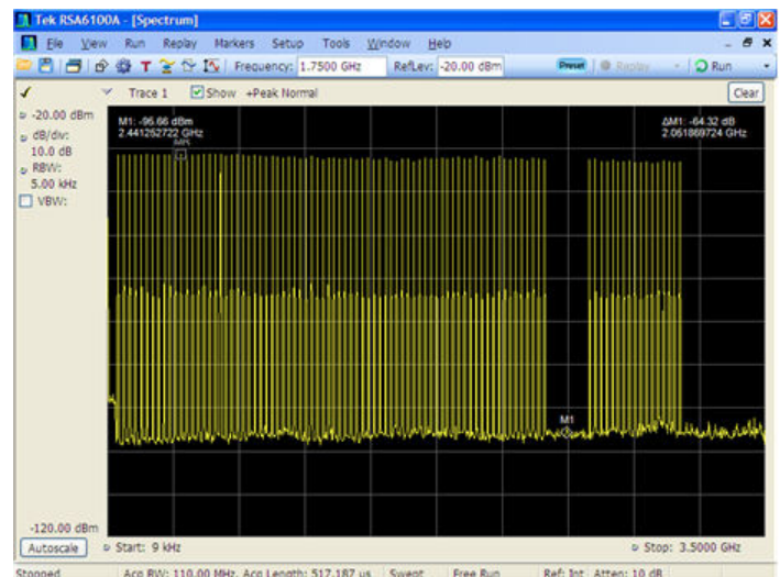
Figure 2: 3 GHz wide multi-carrier signal generated on the AWG70000B with over 60 dBc SFDR
