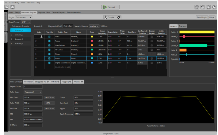
Figure 4: Multiple scenarios with multiple emitters using the Environment plug-in
