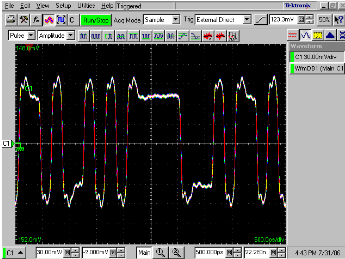
Figure 6: Digital data with de-emphasis added using the AWG7000B and the HSS plug-in
