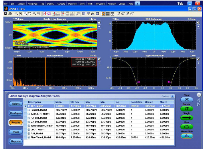
Figure 5: Easily create digital data impairments with the AWG70000B and HSS plug-in
