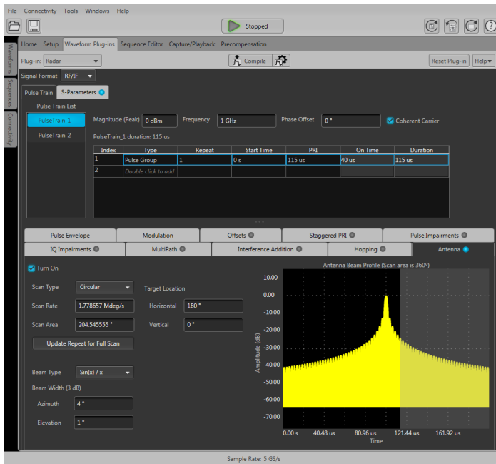
Figure 3: AWG radar pulses created with AWG70000B and Radar plug-in
